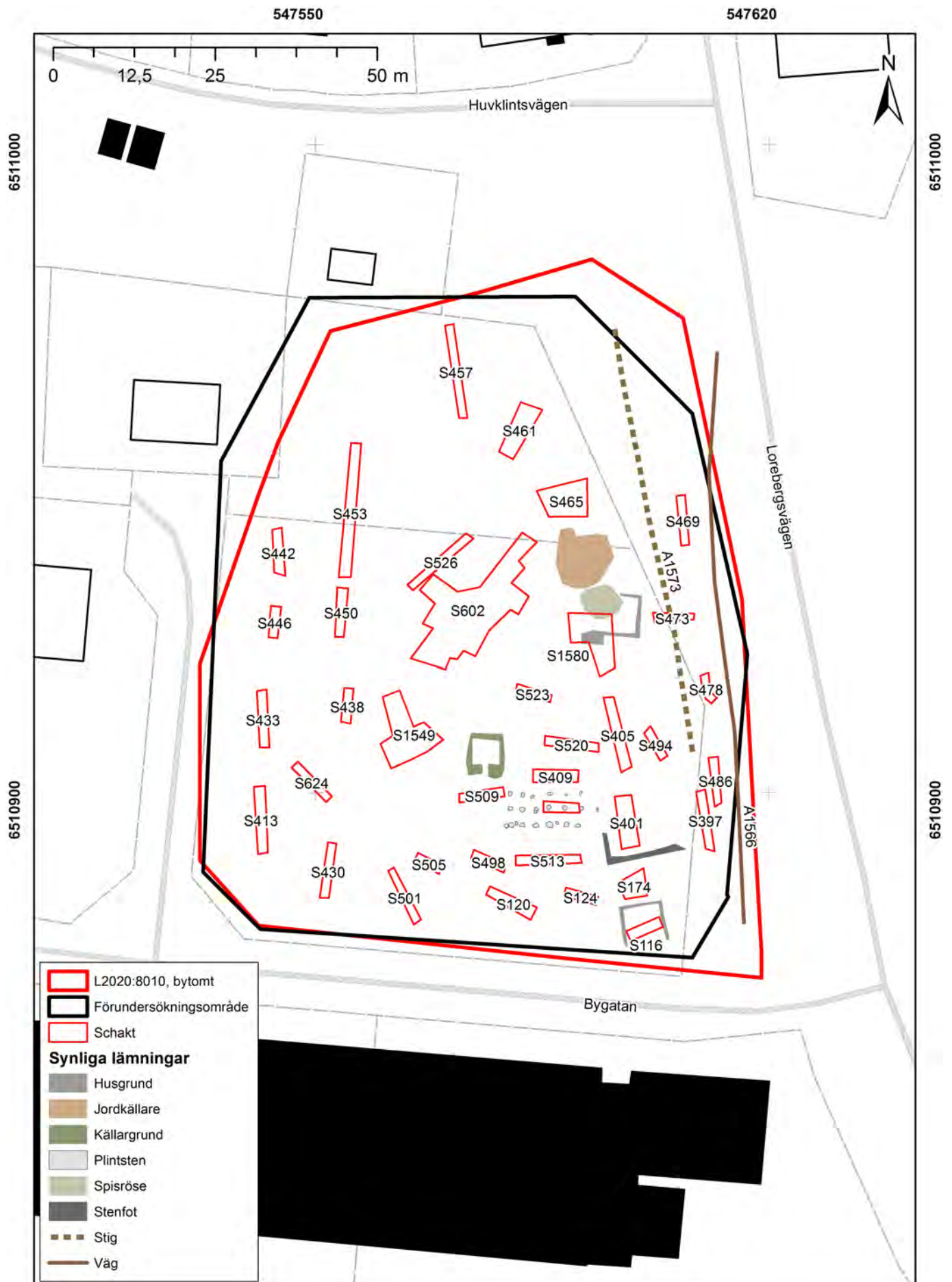
Figur 7. Schaktplan. Skala 1:800.
